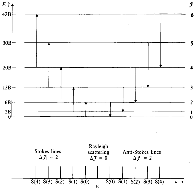
10.6 A Raman spectrum for rotational transitions. The scattered light contains a line at the incident frequency \nu_i due to Rayleigh scattering \Delta J = 0 , and equally spaced lines on either side due to Raman scattering with |\Delta J| = 2 . Transitions with |\Delta J| = 2 are often called the S branch and are numbered by the J value of the lower level.
